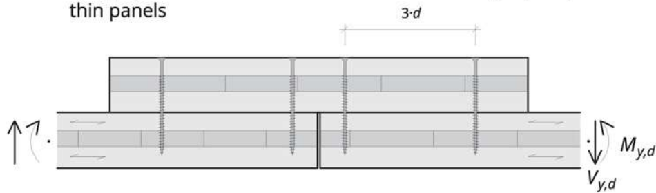
Figure 9-8: Rigid joints
