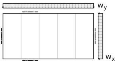
Diaphragm with bracing walls and wind impact
