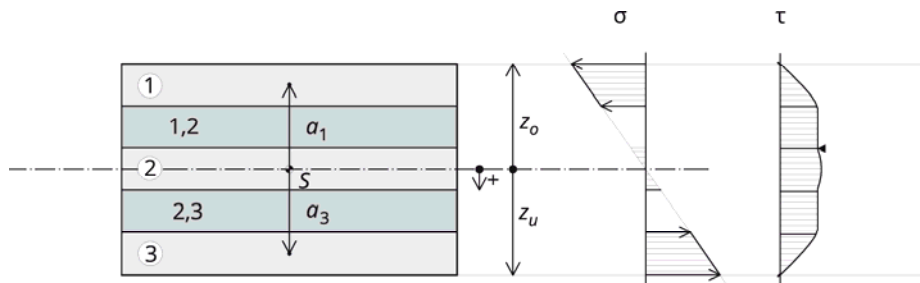
Figure 4-1: Symmetrical cross-section: designation of layers and dimensions
