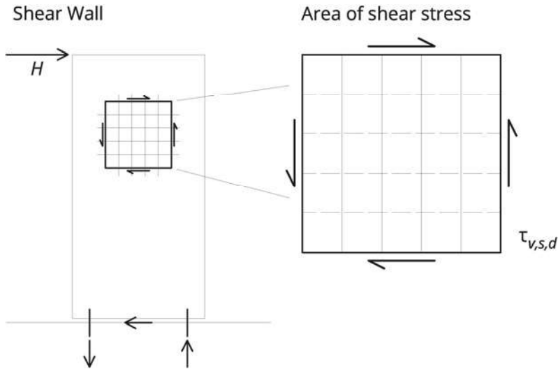
Figure 5-13: Shear within a shear wall
