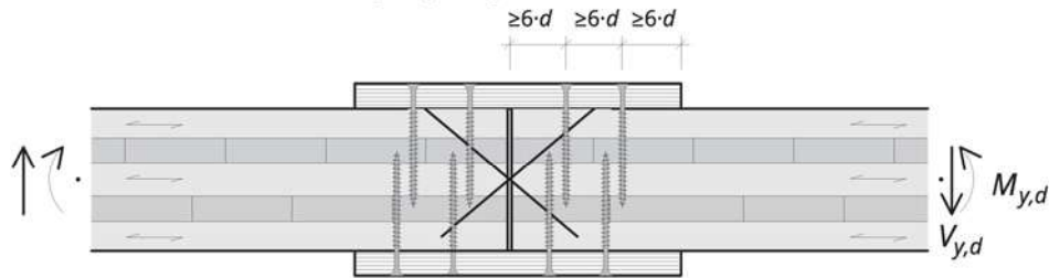
a) Rigid joint in the main direction of load-bearing capacity
