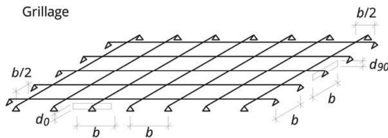
Figure 4-8: Grillage model
