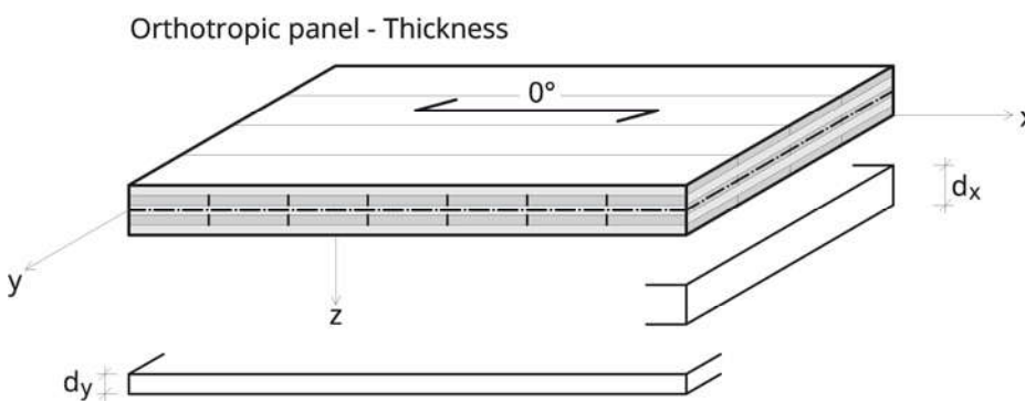
Figure 4-4: Substitute thicknesses for orthotropic panels
