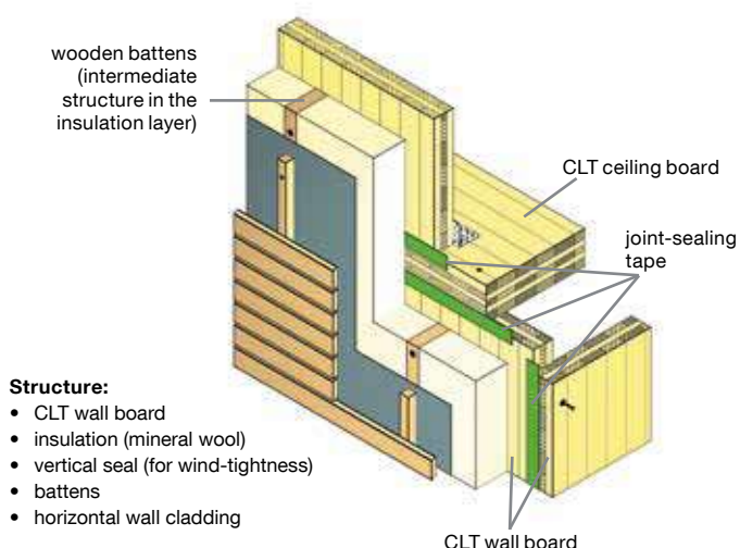
External wall Insulation with mineral wool
