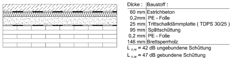
Figure 36: Impact of non-bonded granular material on weighted standard impact sound insulation L_{n,w} , source: [Ferk 2006]
