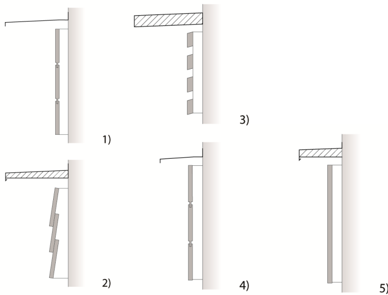
Figure 99: Execution of fire protection barriers (numbers correspond to Table 32)
