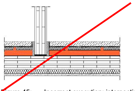
Figure 45: Incorrect execution: intersection of pipelines
