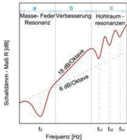
Figure 20: Sound reduction index of double-leaf components
