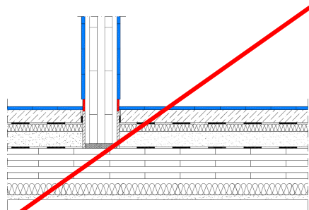
Figure 68: Joint filler between wall and floor tiles
