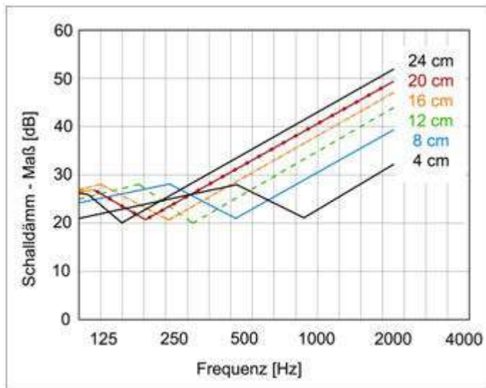
Figure 21: Calculated sound insulation index of jointless solid timber slabs depending on their thicknesses, source: [Bednar et al. 2000]
