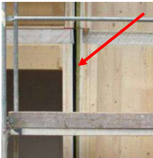
Figure 35: Stone wool and inadmissible continuous air layer between partition walls
