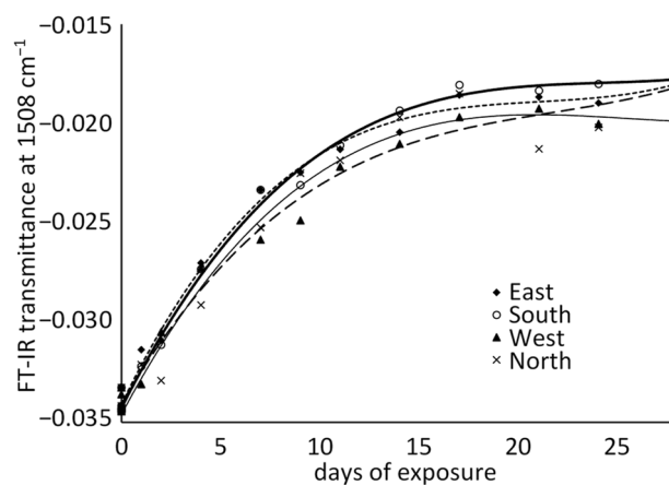
Figure 9. Changes to FT-IR lignin peak ( 1508\text{ cm}^{-1} ) along the natural weathering test duration in samples exposed to diverse cardinal directions.
