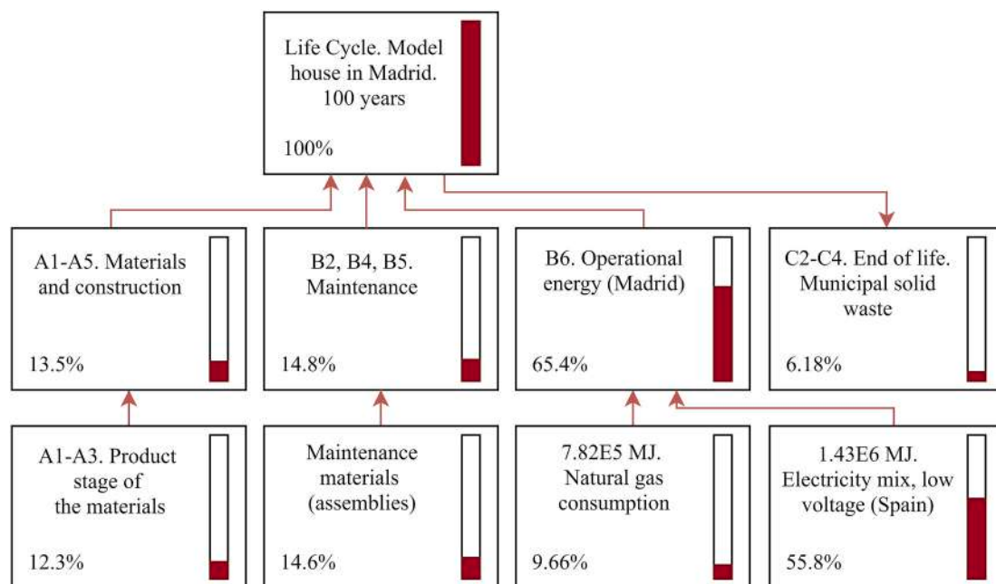
Fig. 7. Contribution of each module to the total carbon emissions in Portorož.
