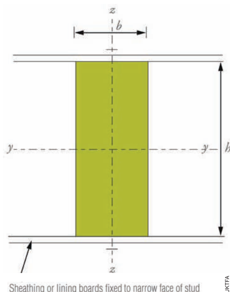
Figure 8 Wall stud plan view and nomenclature
