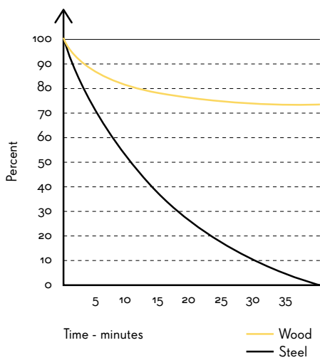
WOOD VS STEEL: LOSS OF STRENGTH IN FIRE
