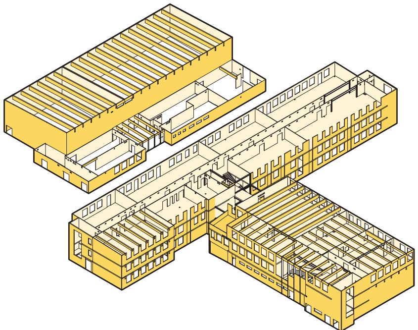
Sectional Axonometric of CLT
