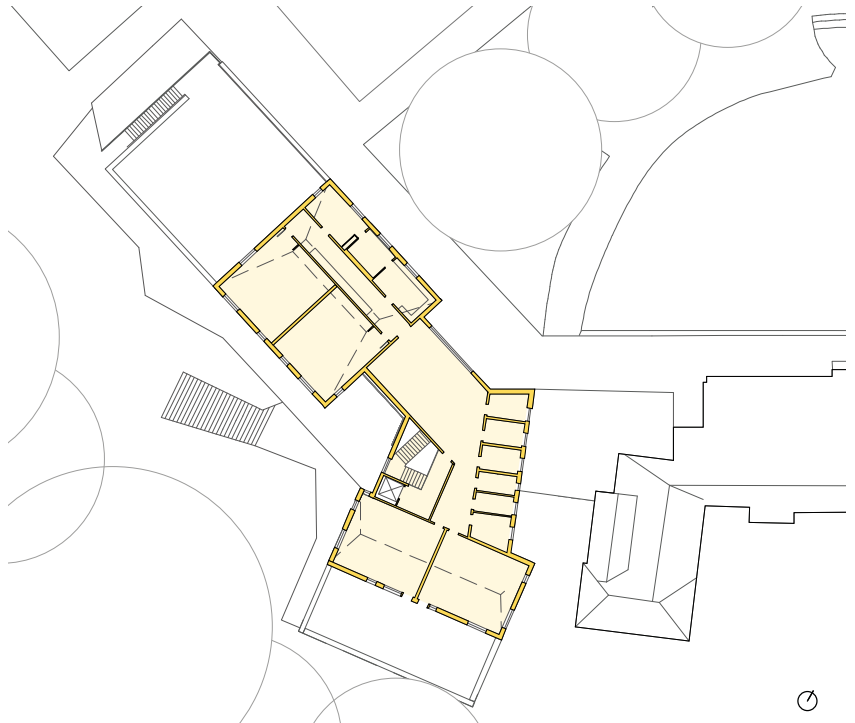
First Floor Plan in Context
