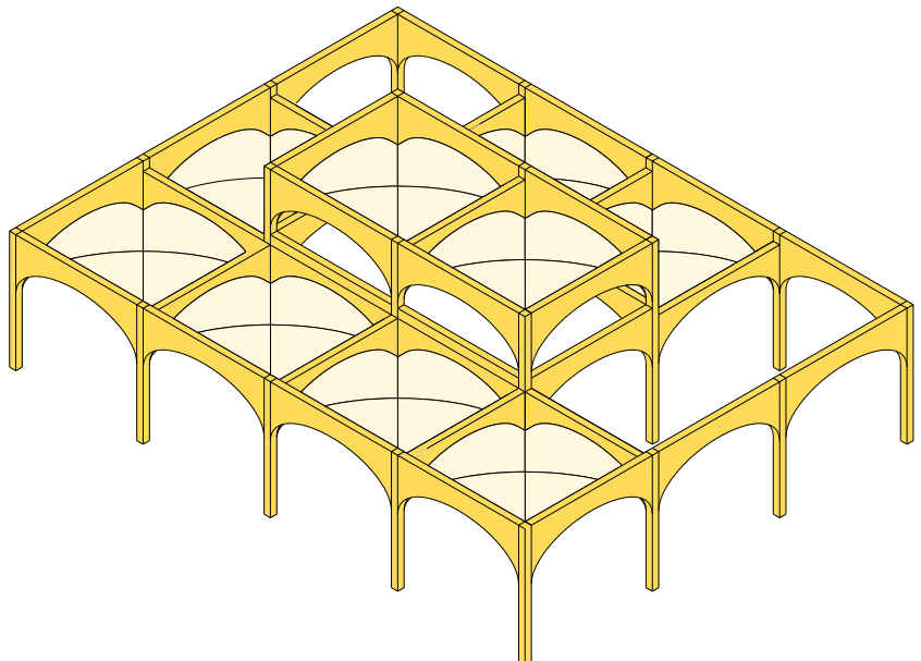
Axonometric Structural Diagram
