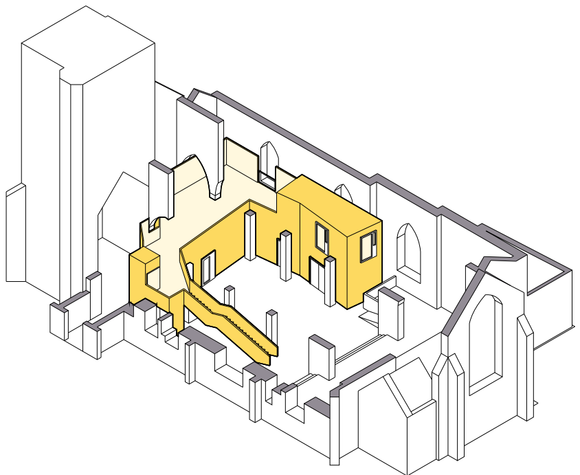
Sectional Axonometric
