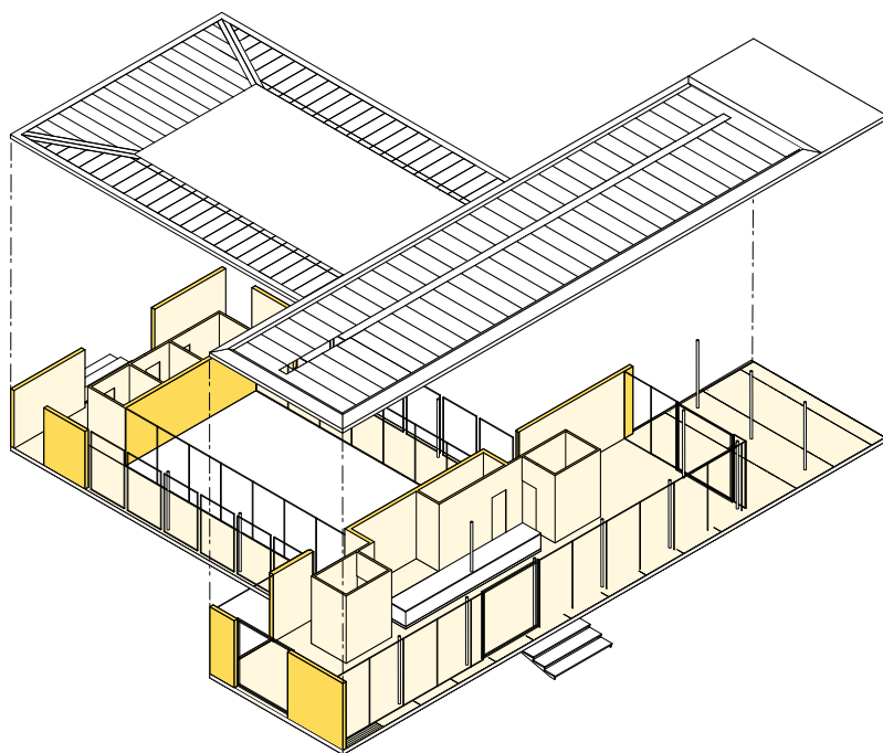
Exploded Axonometric
