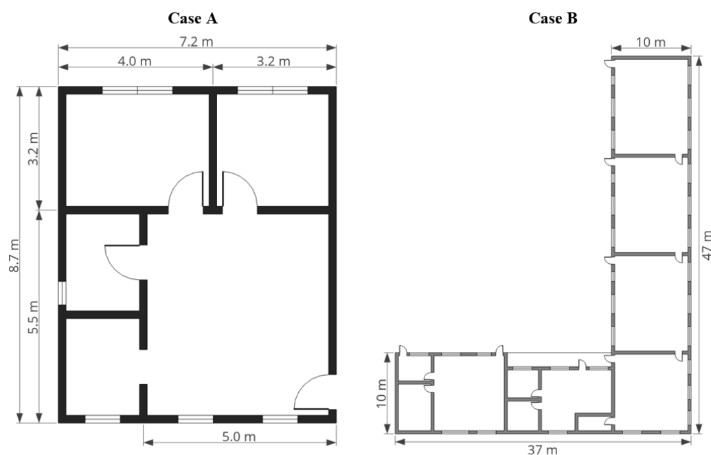
Figure 2. Floor plans of Case A: a granny flat with 63 m 2 area; and Case B: a three-story school with 740 m 2 per storey.
