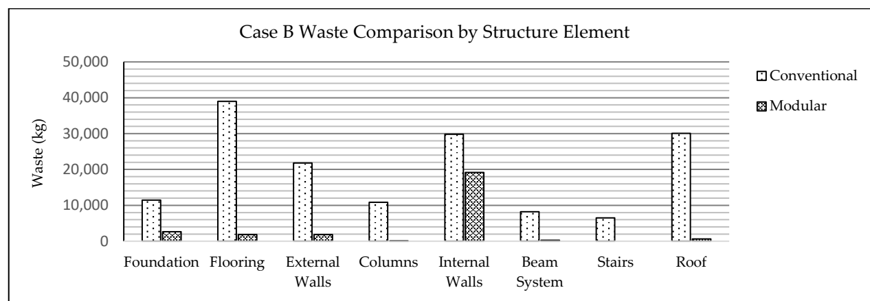
Figure 4. Case B waste comparison by structure element.
