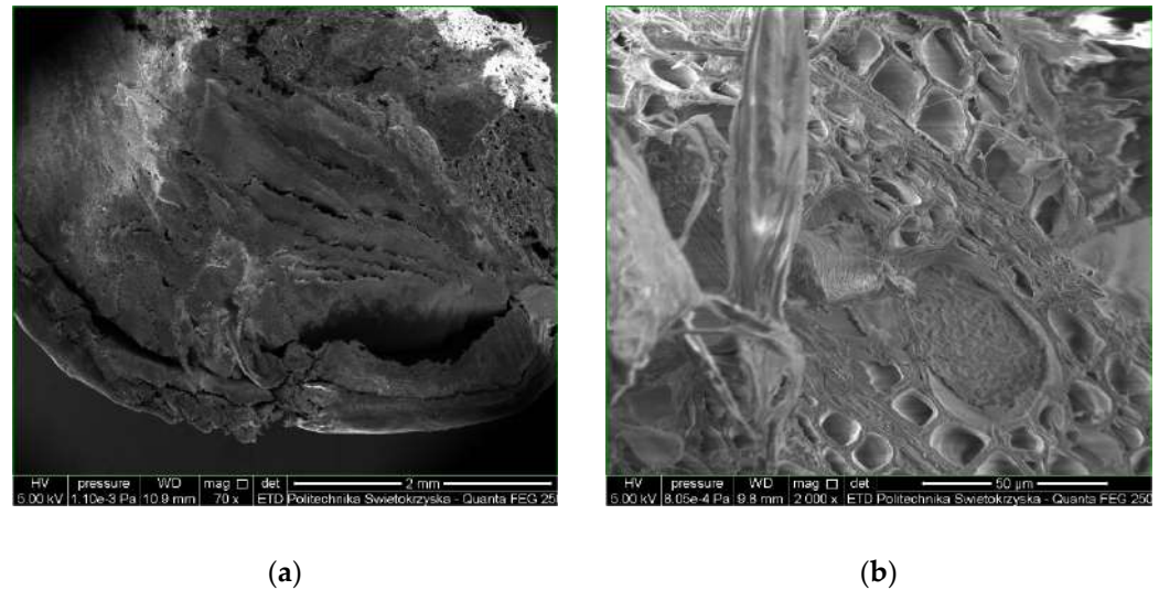
Figure 13. Scanning electron microscope (SEM) images of wood: (a) wet wood, horizontal cross section, magnification 70\times ; and (b) wet wood, vertical section, magnification 2 \times 10^3 .
