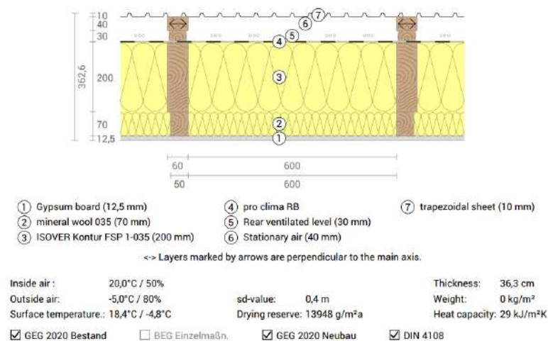
Figure 26. Cross section through the roof layers in a frame building.
