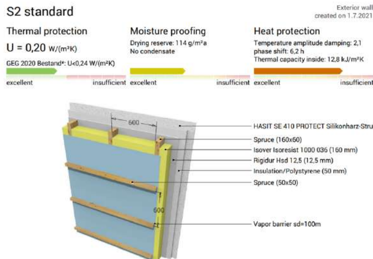
Figure 23. A section through a wall in a standard frame building.
