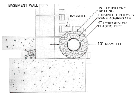
Figure 7: Prefabricated drainage system, using EPS chips instead of gravel.
